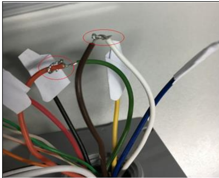
Figure 79: Wiegand Cable Connection
