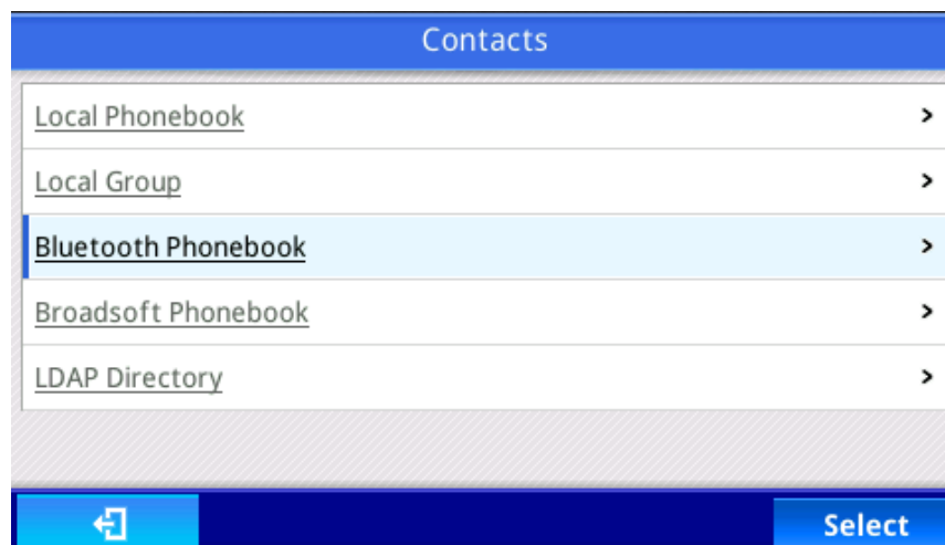
Figure 11: Bluetooth Phonebook
