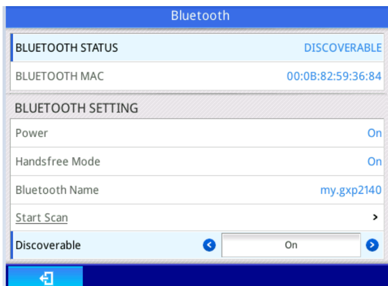
Figure 1: Bluetooth Configuration
