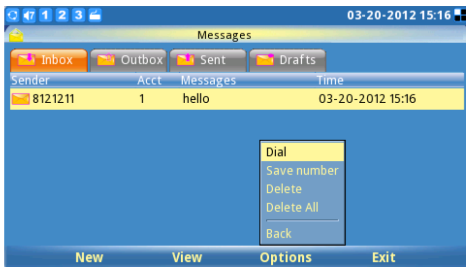
Figure 15: Message Screen
