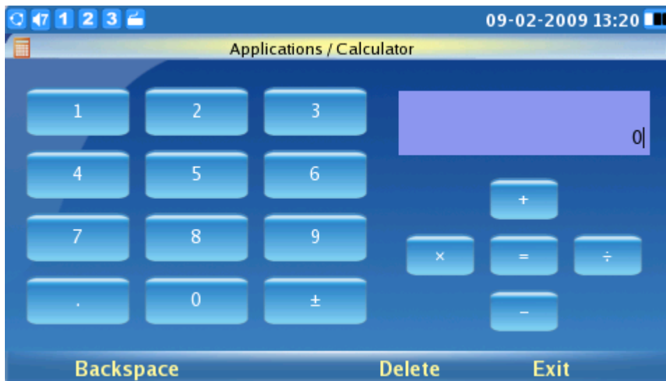
Figure 108: Calculator Application
