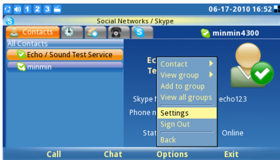
Figure 37: Skype Settings
