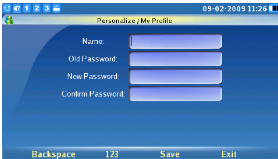
Figure 146: Profile Settings
