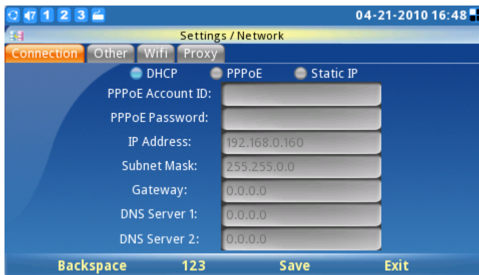
Figure 123: Network Settings
