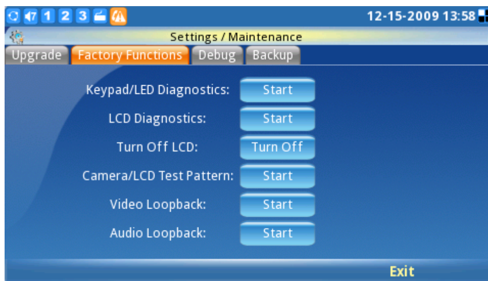
Figure 132: Factory Functions
